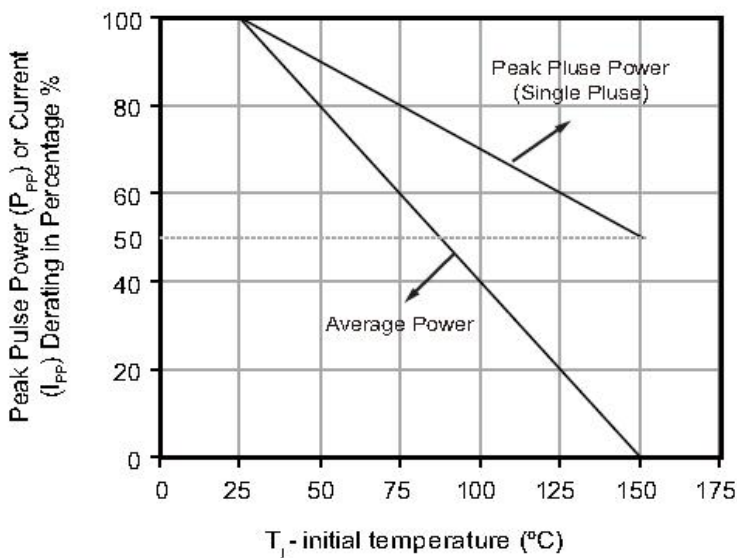
Fig.3 Peak Pulse Power or Current Derating
